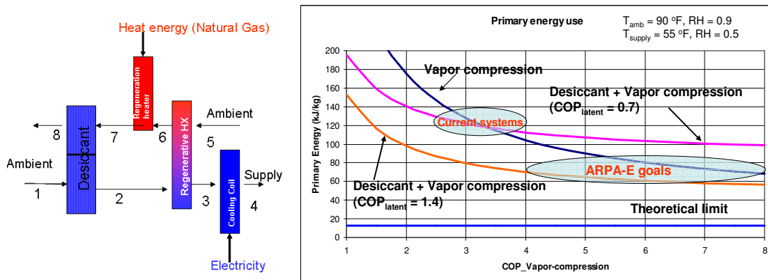
Fig. 2 (Left) A desiccant-based cooling system with regenerative heat exchange. In an ideal system the heat exchange should have an effectiveness of 1 and the desiccant should have no hysteresis during sorption-desorption cycles. (Right) Primary energy input as a function of COP of the vapor compression system for a particular set of ambient and supply conditions. Also shown is an ideal system operating at thermodynamic limit, the current systems and ARPA-E target for the current FOA.
