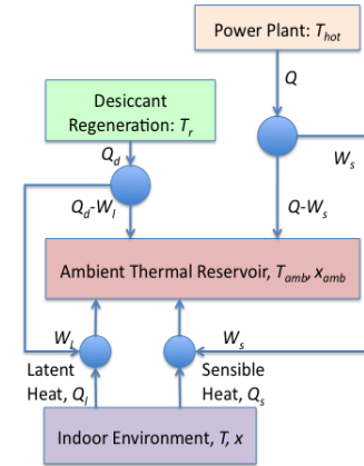
Fig. 1 Schematic diagram showing ideal system with Carnot engines and refrigerators. Note that (Q_d + Q) is the minimum primary energy input.
